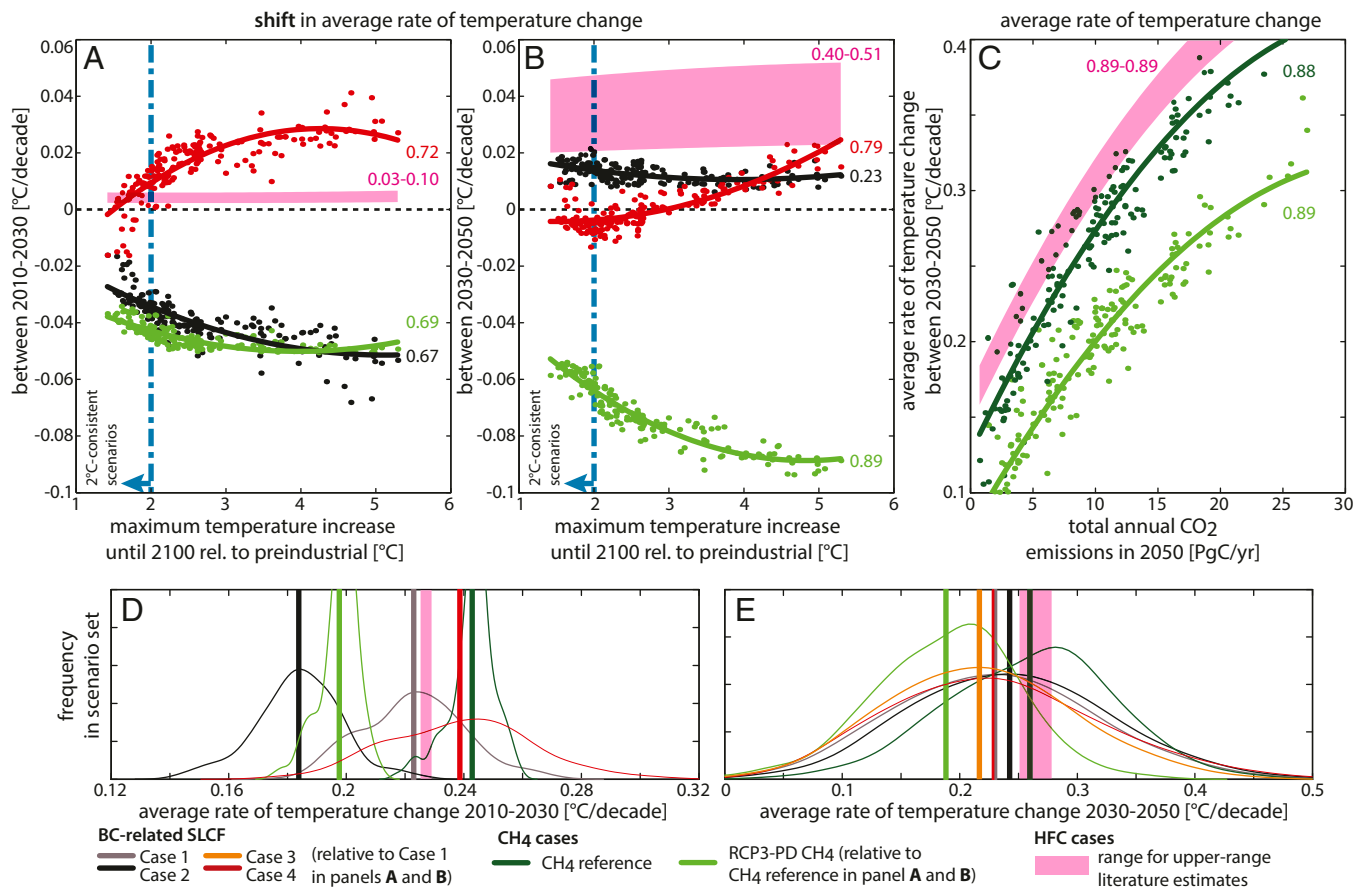
Fig. 3. Influence of SLCF and CO 2 mitigation on ARTCs between 2010–2030 (A) and 2030–2050 (B) as a function of maximum warming until 2100 relative to preindustrial levels under the reference scenario (Case 1). (C) ARTCs between 2030–2050 as a function of CO 2 emissions in 2050. (D and E) Frequency distributions of ARTCs between 2010–2030 and 2030–2050, respectively, together with mean estimates (vertical solid lines) over the entire ensemble. Each dot represents the median response per scenario. Solid lines and numbers in A–C are quadratic fits and associated R 2 values for each case, respectively. Pink ranges in A–C are defined by the quadratic fits for the range of HFC estimates. Additional cases are shown in SI Appendix, Figs. S8 and S9 .
