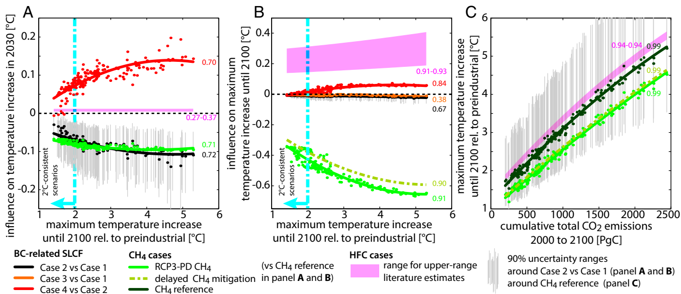
Fig. 2. Influence of various SLCF measures on global-mean warming by 2030 ( A ) and on maximum warming until 2100 ( B ), as a function of maximum warming until 2100 relative to preindustrial levels under the reference scenario (Case 1). ( C ) Maximum temperature increase until 2100 as a function of cumulative CO 2 emissions between 2000 and 2100. Scenarios at the left of the “2 °C-consistent scenarios” line limit warming to below 2 °C with at least 50% probability. The effect of SLCF measures is smaller in stringent CO 2 mitigation scenarios. Variation along each colored line is entirely driven by CO 2 mitigation and technological SLCF linkages. Dots represent the median response per scenario (vertical gray lines: 90% range). Solid lines and numbers are quadratic fits and associated R 2 values for each case, respectively. Pink ranges are defined by the quadratic fits for the HFC estimates. Additional cases and metrics are shown in SI Appendix, Figs. S4–S6 .
