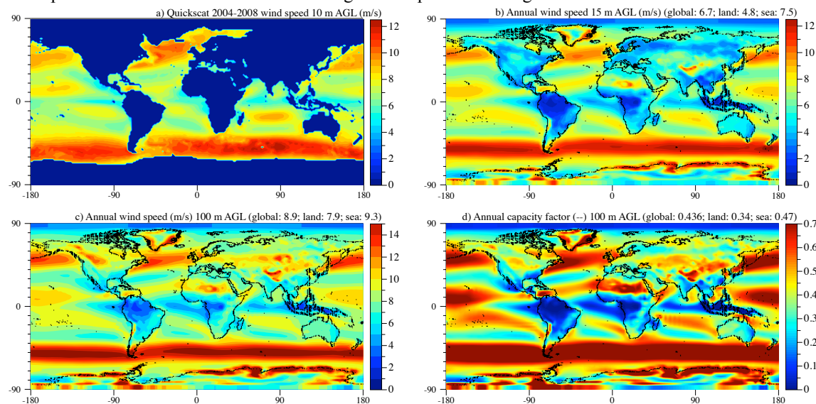
Figure S3. (a) QuikSCAT 10-m above ground level (AGL) wind speed at 1.5^\circ \times 1.5^\circ resolution (JPL, 2010), (b) GATOR-GCMOM (Jacobson et al., 2007; Jacobson, 2010a,b; Ten Hoeve et al., 2012) 4-year-average modeled annual 15-m AGL wind speed at 2.5^\circ W-E \times 2.0^\circ S-N resolution, (c) Same as (b) but at 100 m AGL, (d) Same as (c) but showing capacity factors assuming a Senvion (RePower) 5 MW turbine with 126-m rotor diameter. In all cases, wind speeds are determined before accounting for competition among wind turbines for the same kinetic energy.
