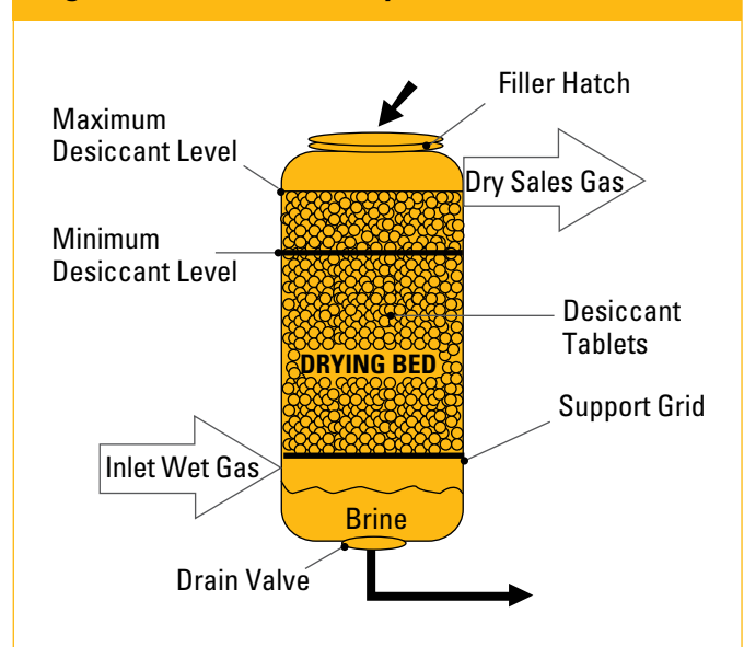
Figure 18: Desiccant Dehydrator Schematic
