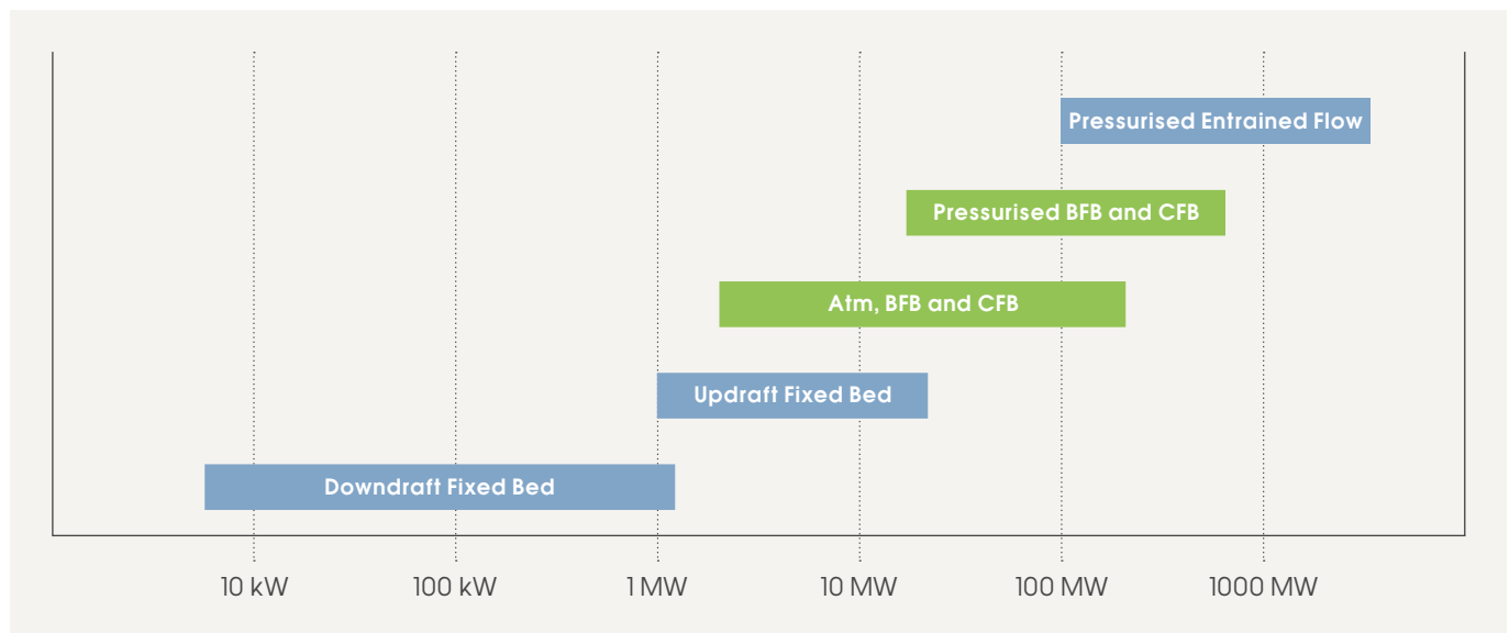
FIGURE 2.5: GASIFIER SIZE BY TYPE
