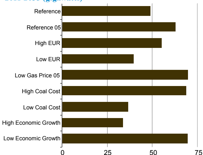
Figure 5. Cumulative retirements of coal-fired generating capacity by NERC region in nine cases, 2011-2035 (gigawatts)
