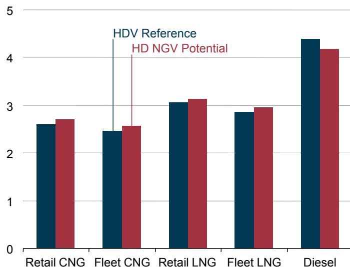
Figure 40. Diesel and natural gas transportation fuel prices in two cases, 2035 (dollars per diesel gallon equivalent)
