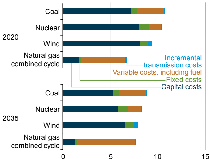
Figure 98. Levelized electricity costs for new power plants, excluding subsidies, 2020 and 2035 (2010 cents per kilowatthour)
