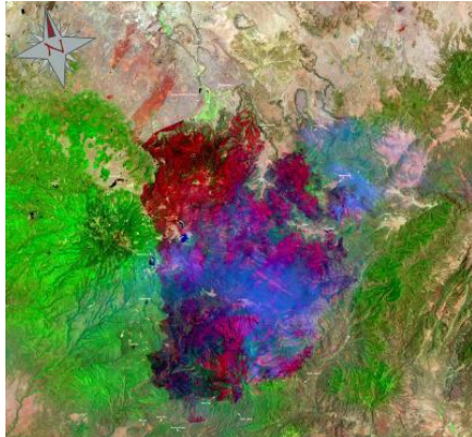
Figure 6-1. Landsat 5 Satellite Image of the Wallow North Fire in East Central Arizona (6/15/11).
