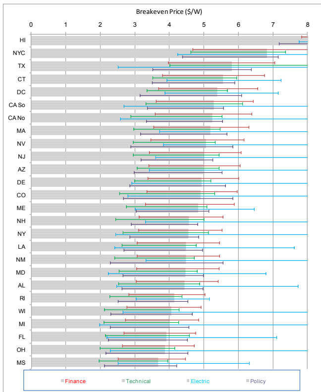
Fig. 3a. Range of PV break-even costs in the 2015 scenarios: Top 26 regions
