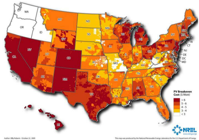
Fig. 2: Residential solar PV break-even cost ($/W) in 2015 using the base-case assumptions in Table 1 and an optional time-of-use rate in all states
