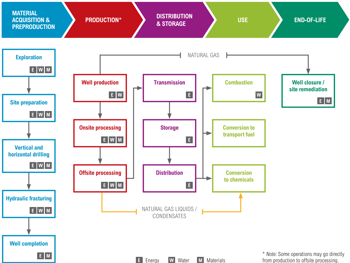
Figure 1 | The WRI life cycle process map includes life cycle stages and attributable processes
