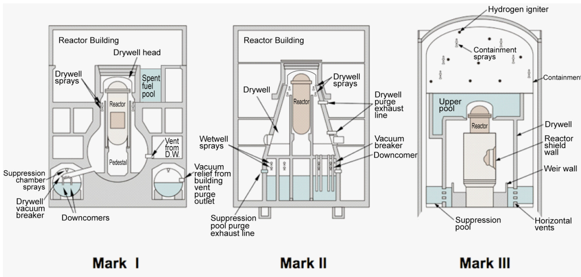
Figure 6. Generations of BWR containments.
