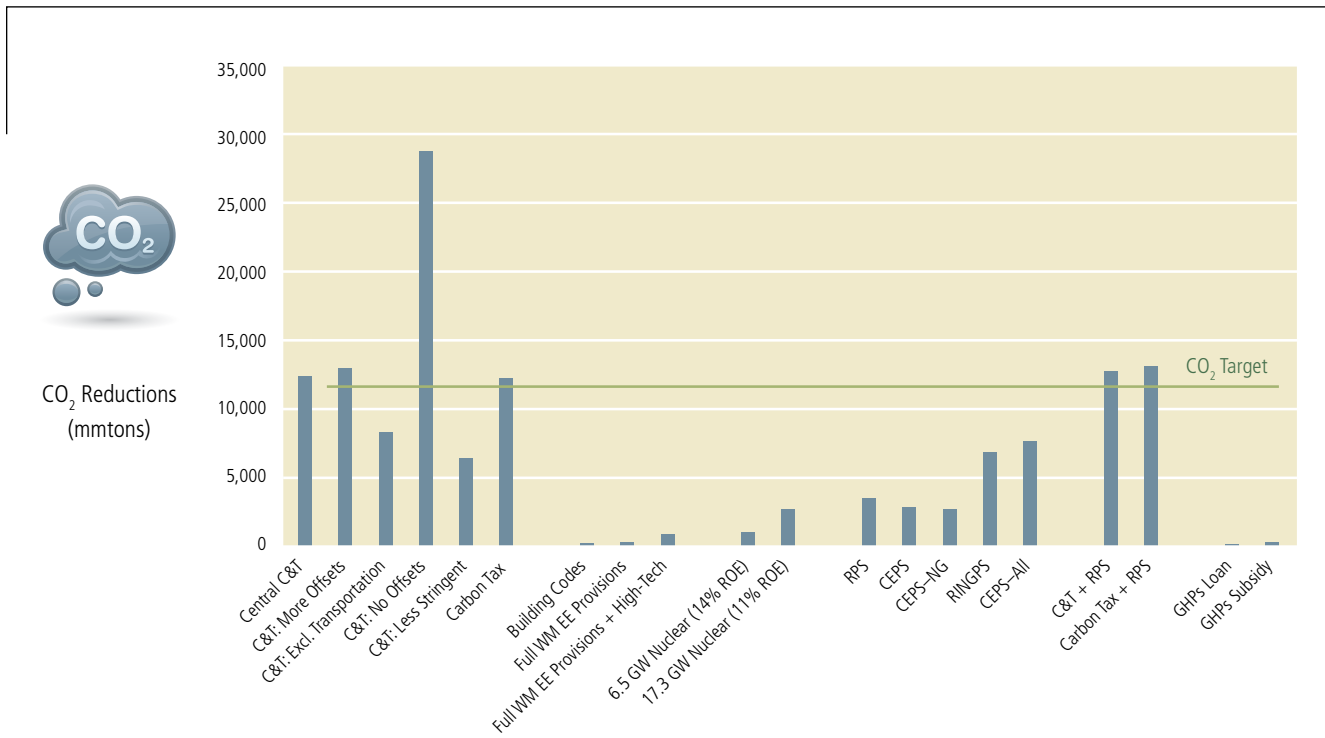
Figure 6.13: Cumulative Reductions in CO 2 Emissions Relative to the Reference Case, 2010–2030
