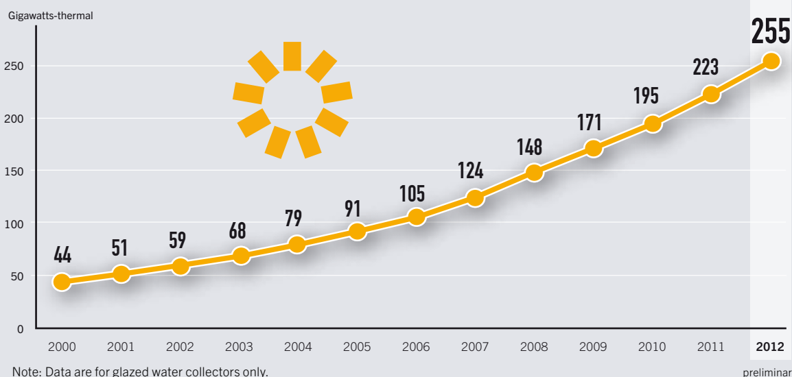
FIGURE 17. SOLAR WATER HEATING GLOBAL CAPACITY, 2000–2012
