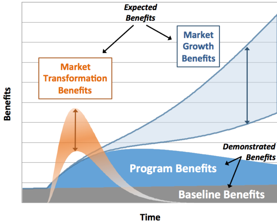
Figure E-1: General Types of Benefits as a Function of Time
