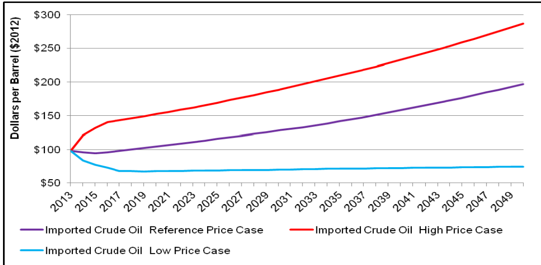
Figure 32: Crude Oil Price Cases
