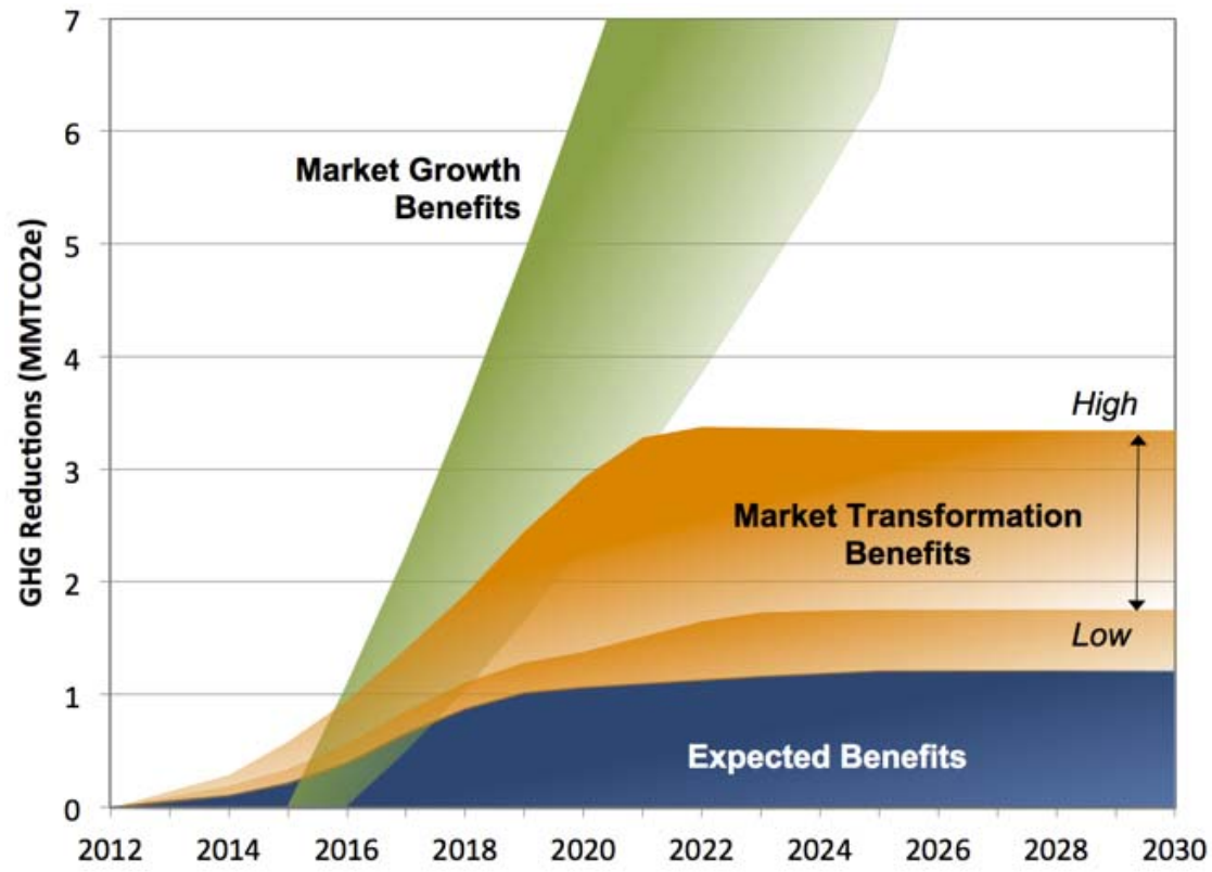
Figure 24: Expected and Market Transformation Benefits in Context of Market Growth Benefits Needed to Meet Vision for Clean Air GHG Reduction Goals
