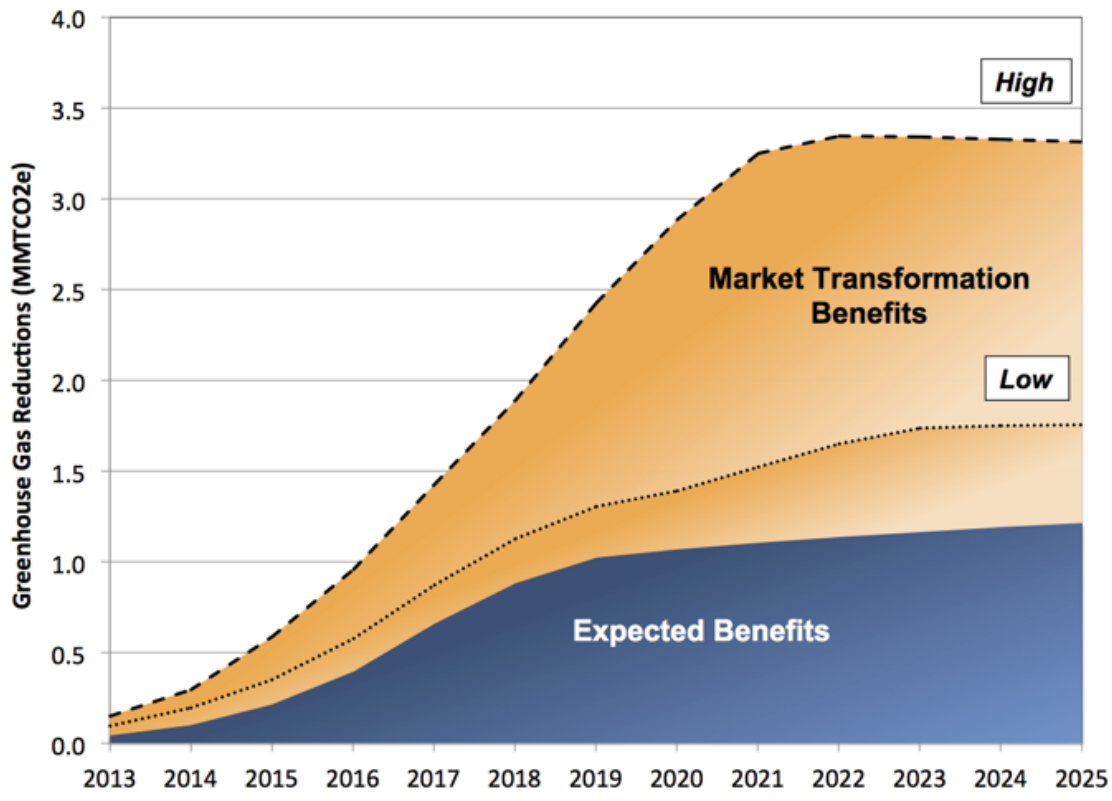
Figure 23: Market Transformation GHG Reduction Benefits Combined with Expected GHG Reduction Benefits through 2025
