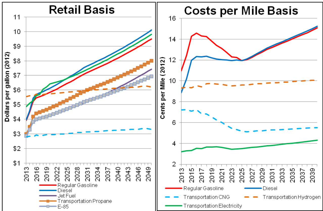
Figure 25: High Energy Price Common Case
