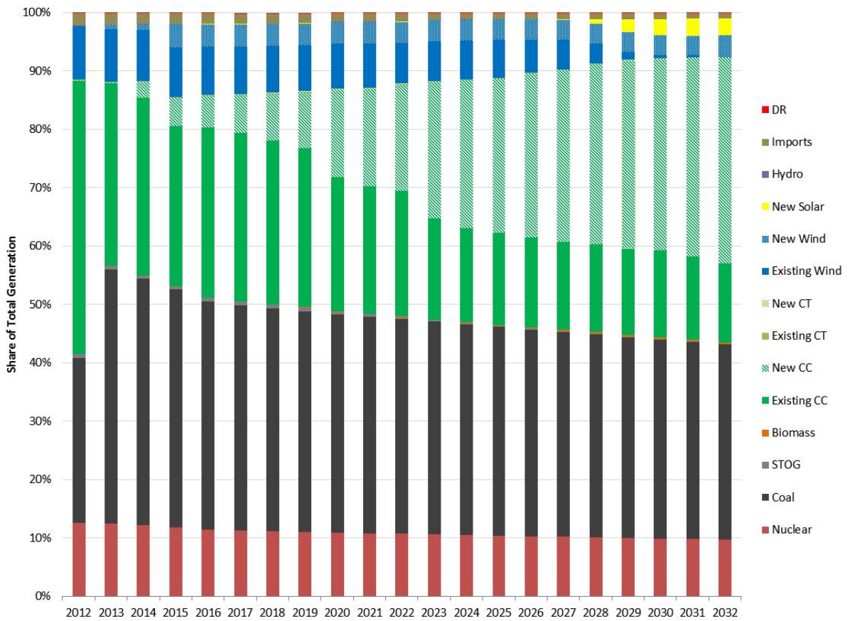
Figure IV-4 Generation Mix by Type Reference Case with Required Reserve Margin
