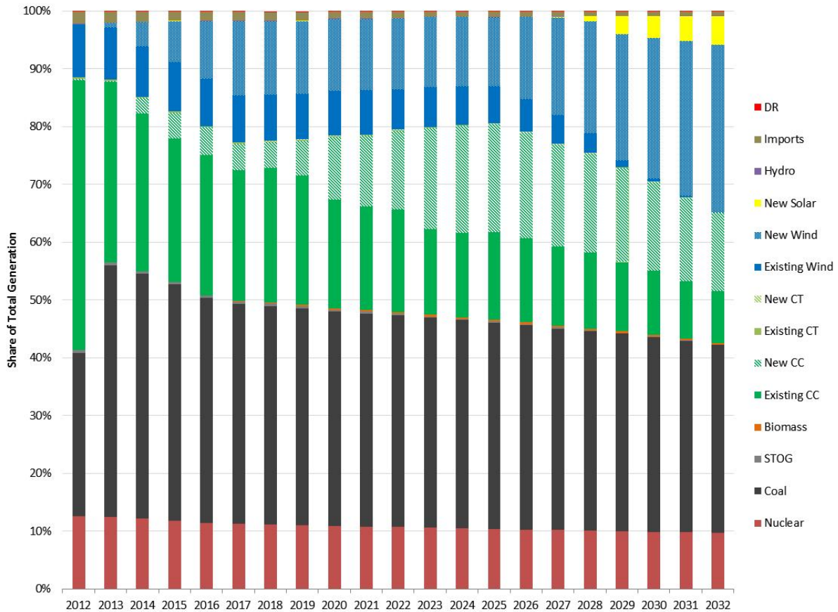
Figure IV-8 Generation Mix by Type High Gas Prices and Low Renewables Costs
