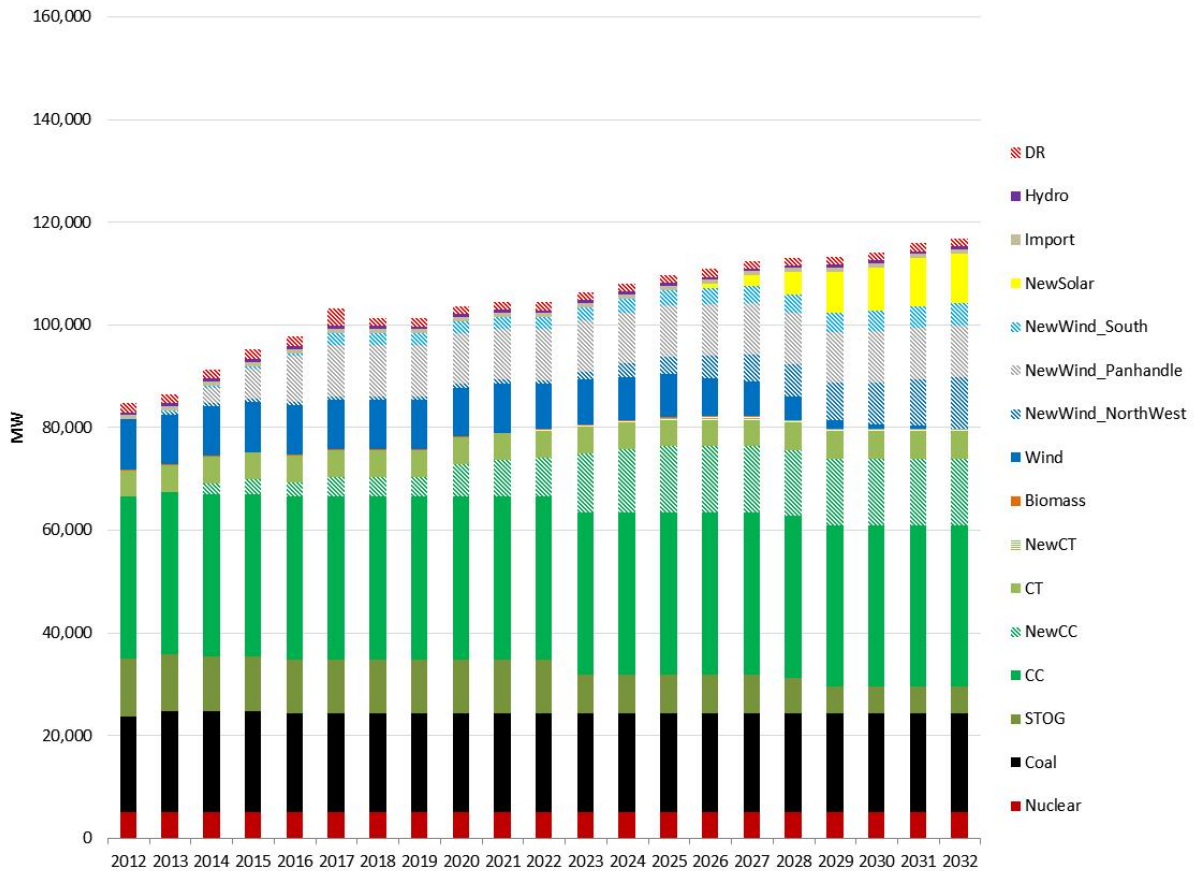
Figure IV-5 Installed Capacity by Type High Gas Prices – No Required Reserve Margin
