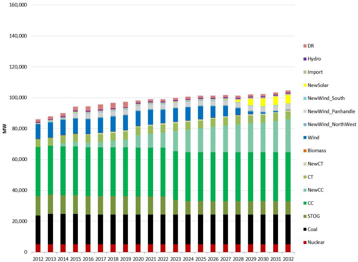
Figure IV-3 Installed Capacity by Type Reference Case With Required Reserve Margin
