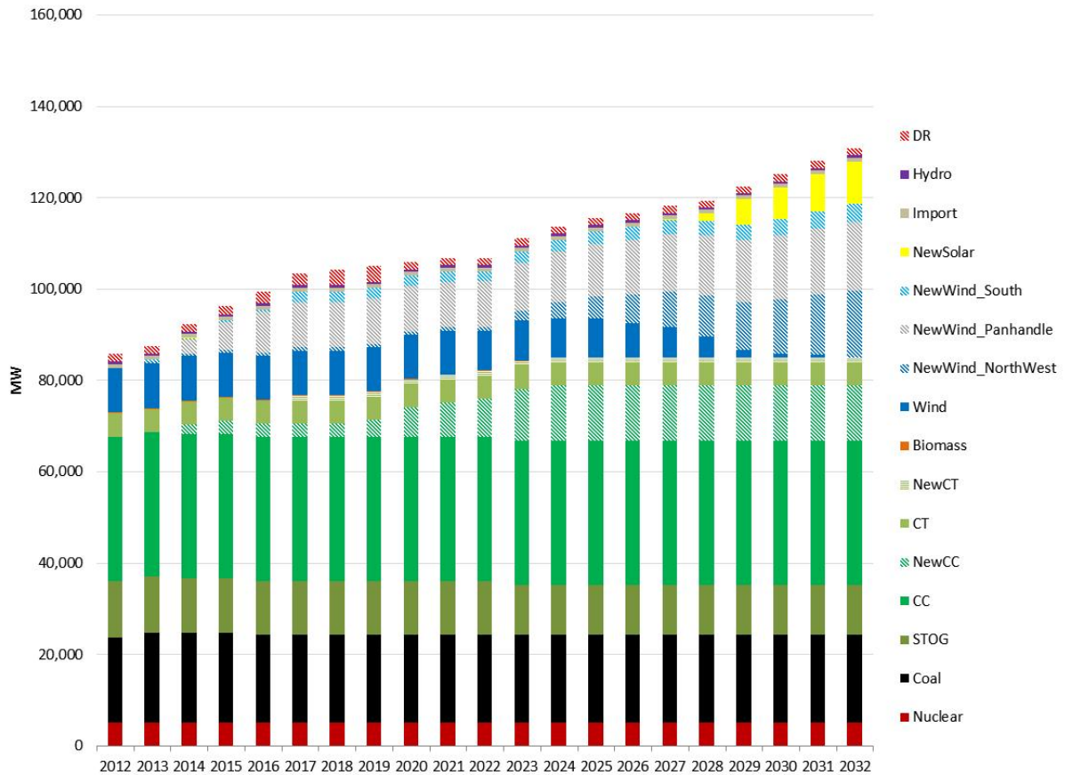
Figure IV-7 Installed Capacity by Type High Gas Prices and Low Renewables Costs
