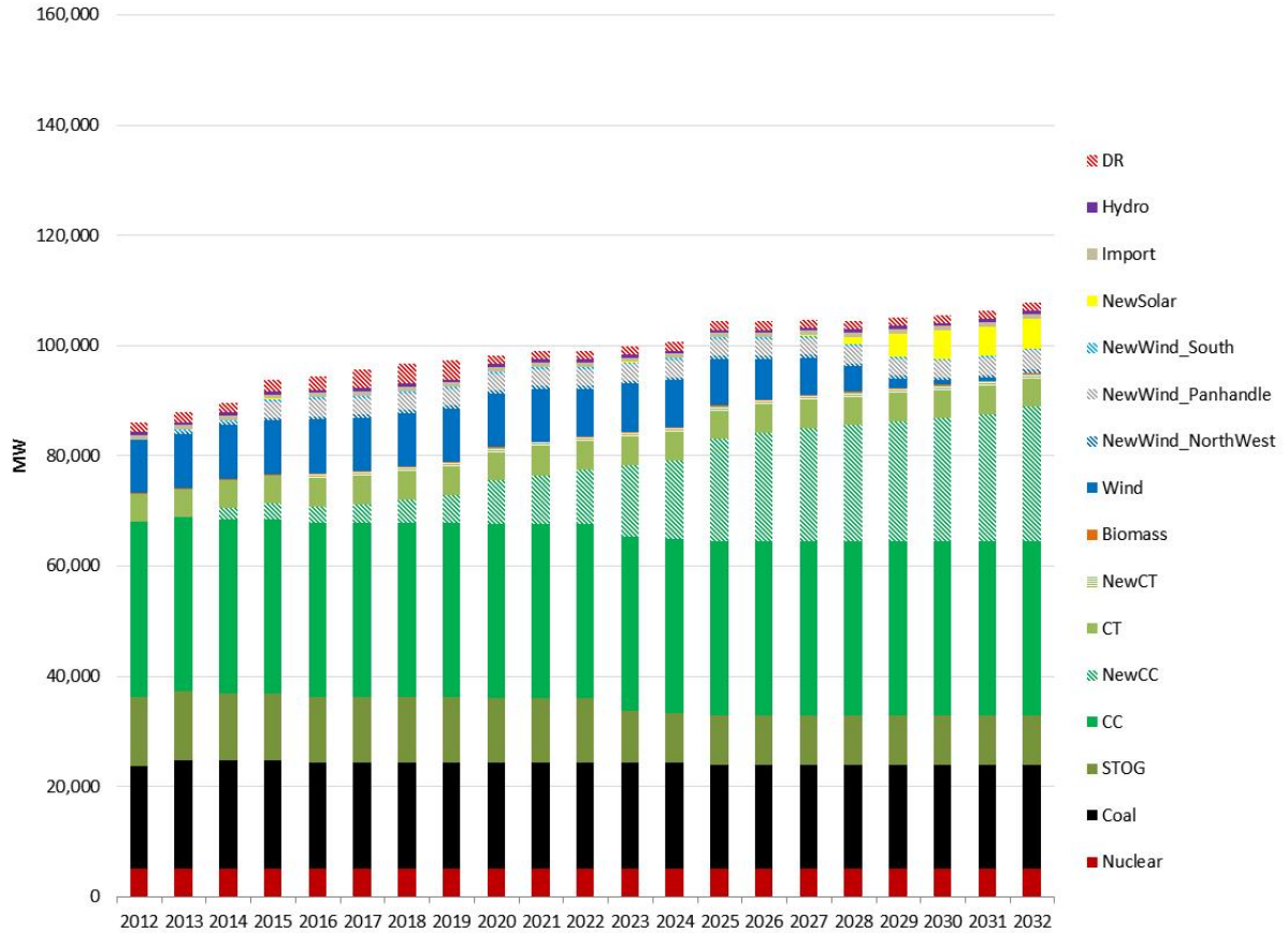
Figure IV-9 Installed Capacity by Type Moderate Federal Carbon Rule with Require Reserve Margin
