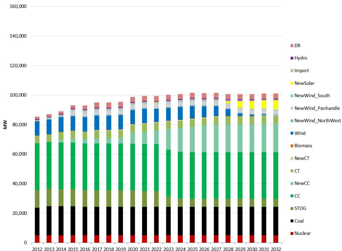
Figure IV-1 Installed Capacity by Type Reference Case without Required Reserve Margin
