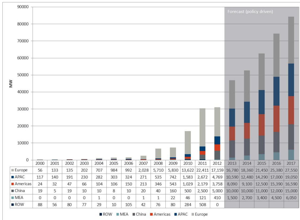
Figure C-2 Annually installed PV capacity in selected regions
