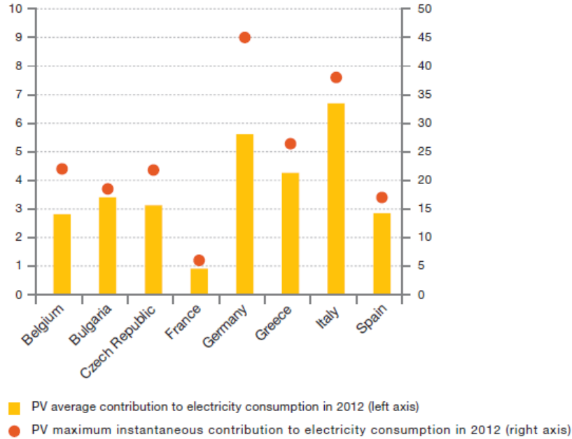
Figure C-5 Annual average and maximum instantaneous PV contribution to electricity consumption in 2012 (%)
