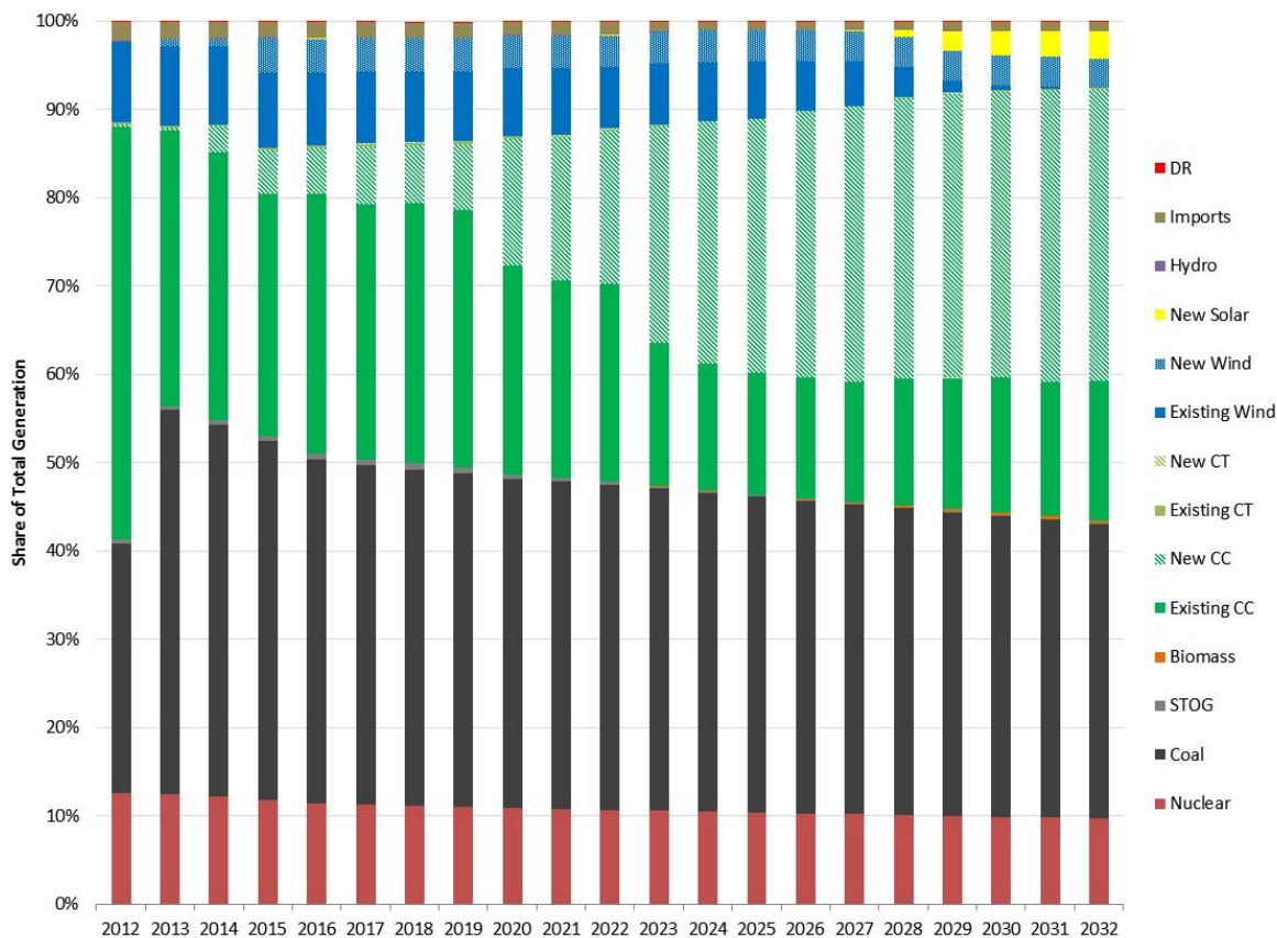
Figure IV-2 Generation Mix by Type Reference Case without Required Reserve Margin
