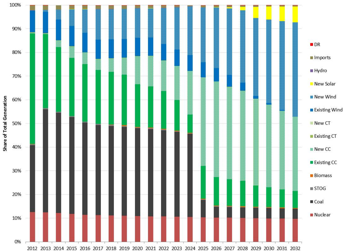
Figure IV-12 Generation Mix by Type Stronger Federal Carbon Rule
