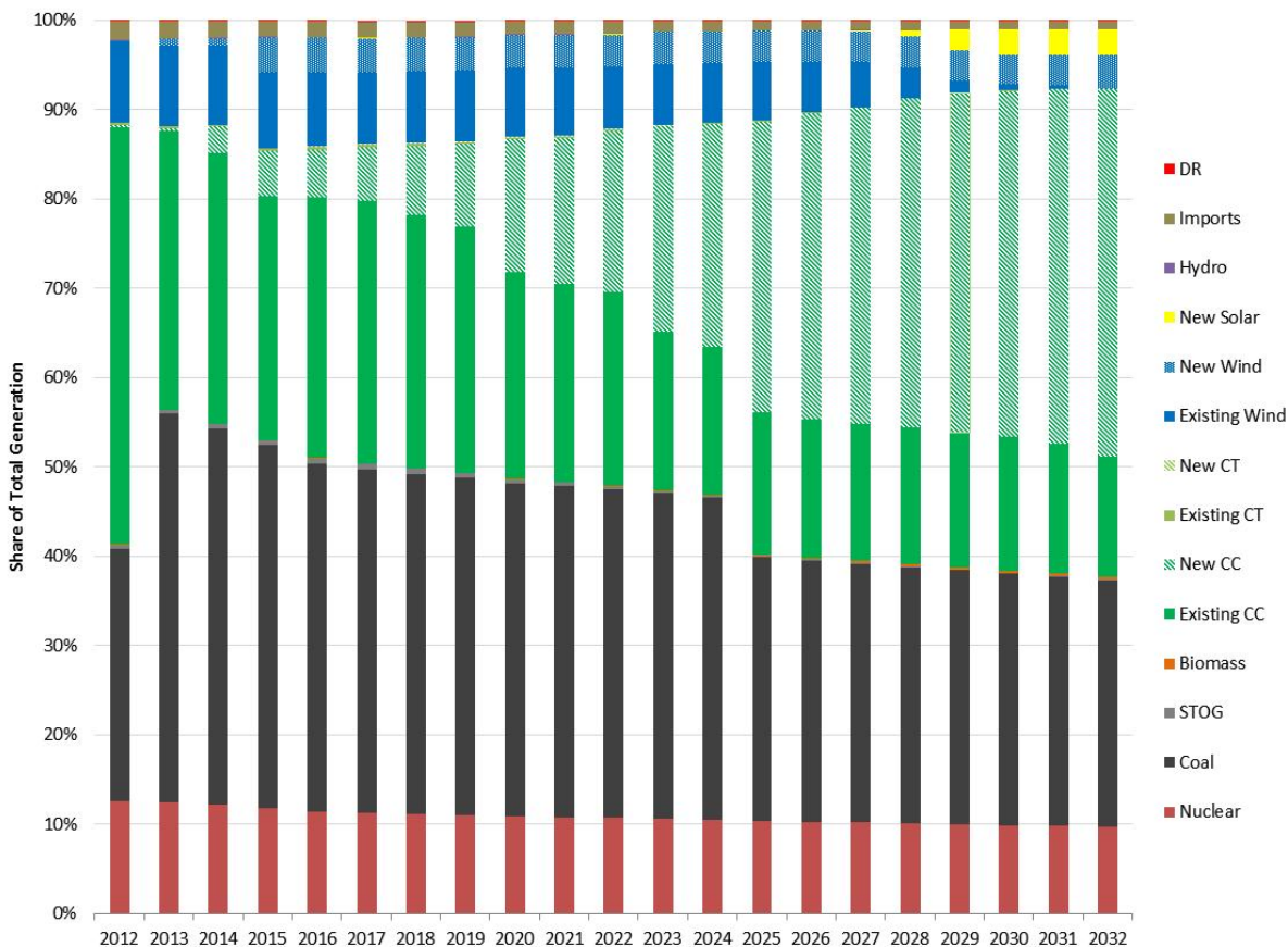
Figure IV-10 Generation Mix by Type Moderate Federal Carbon Rule with Required Reserve Margin
