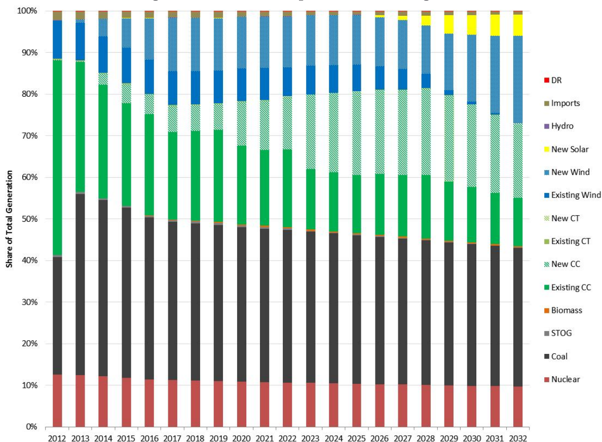
Figure IV-6 Generation Mix by Type High Gas Prices – No Required Reserve Margin
