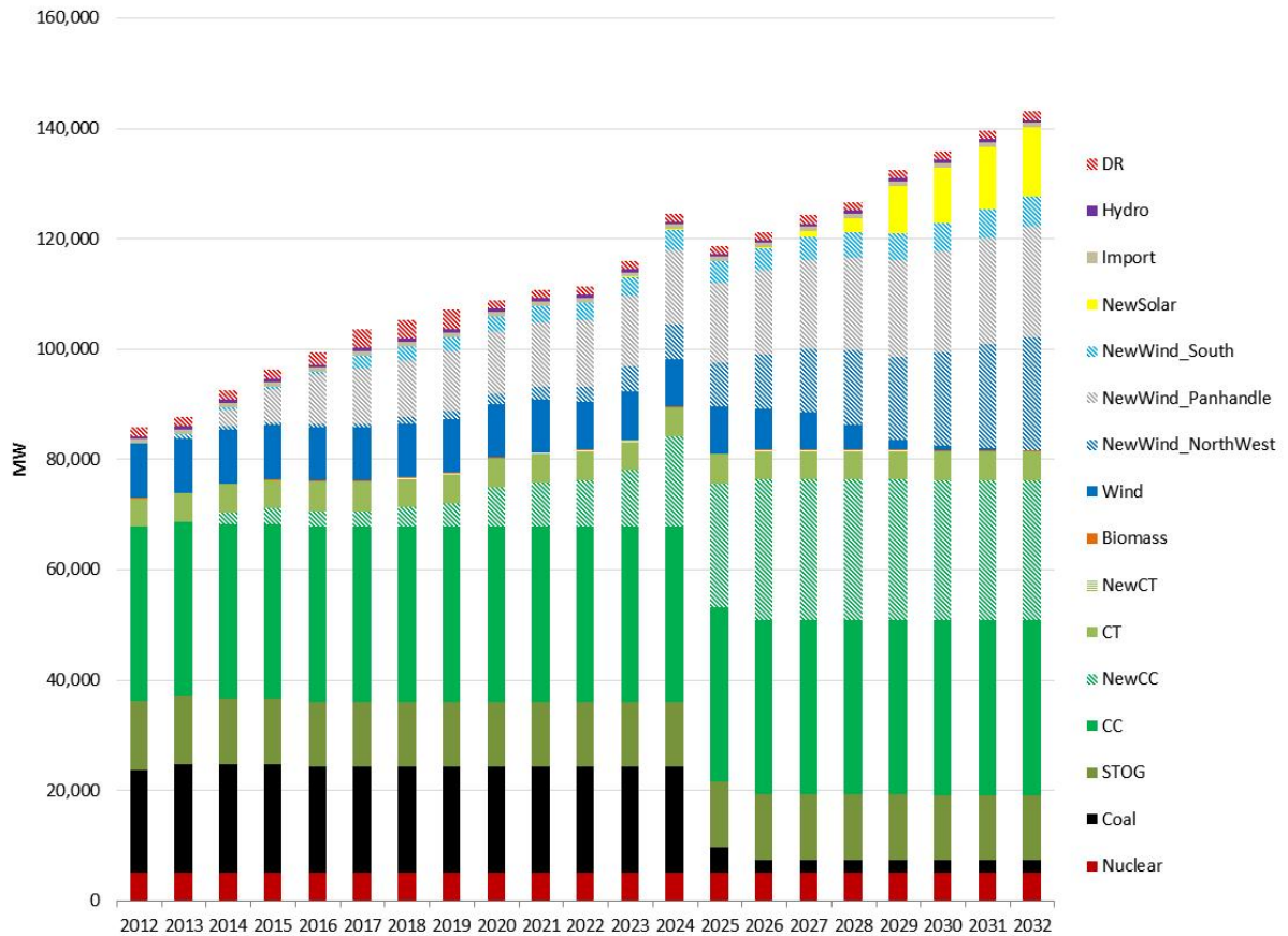
Figure IV-11 Installed Capacity by Type Stronger Federal Carbon Rule
