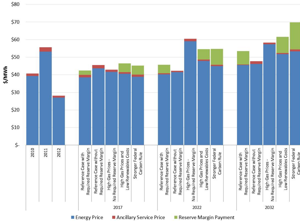
Figure IV-14 Average Annual Wholesale Prices by Component by Scenario
