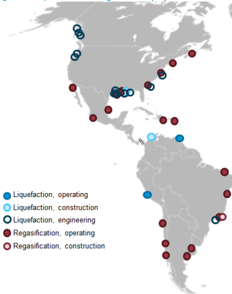
Figure 10. Liquefaction and regasification projects in the Americas
