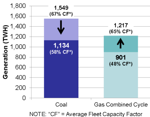
Coal and NGCC Generation in 2020
