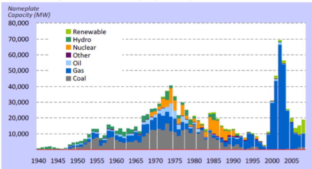
Figure 3: US Electric Generating Capacity by In Service Year
