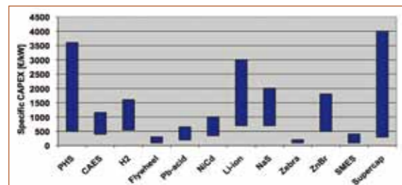
Figure 3: Existing power storage technologies according to their levels of maturity of development, investment costs across different power sectors: generation, transmission and distribution, and end user.
