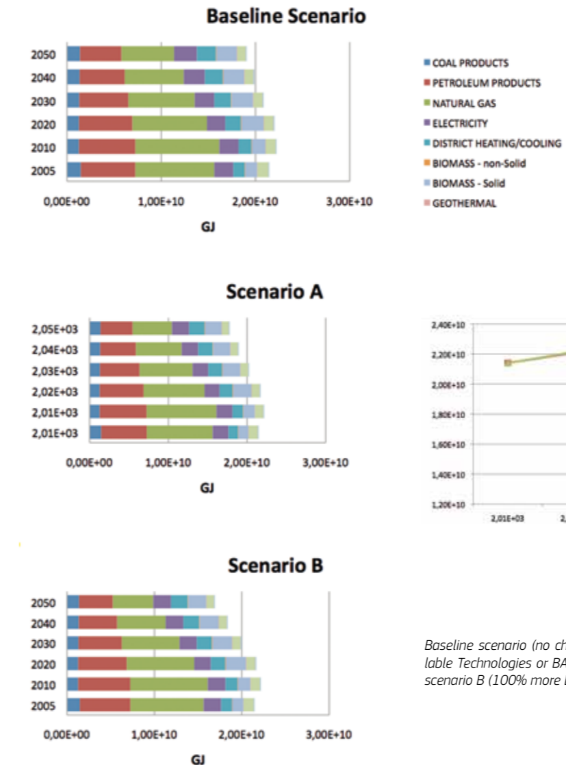
Evolution up to 2050 of the final energy demand for heat in the EU-27
