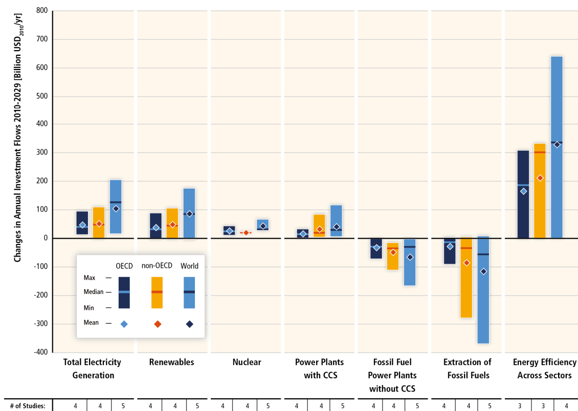
Figure SPM.9. Change in annual investment flows from the average baseline level over the next two decades (2010 to 2029) for mitigation scenarios that stabilize concentrations within the range of approximately 430–530 ppm CO 2 eq by 2100. Investment changes are based on a limited number of model studies and model comparisons. Total electricity generation (leftmost column) is the sum of renewables, nuclear, power plants with CCS and fossil power plants without CCS. The vertical bars indicate the range between minimum and maximum estimate; the horizontal bar indicates the median. Proximity to this median value does not imply higher likelihood because of the different degree of aggregation of model results, the low number of studies available and different assumptions in the different studies considered. The numbers in the bottom row show the total number of studies in the literature used for the assessment. This underscores that investment needs are still an evolving area of research that relatively few studies have examined. [Figure 16.3] [Subject to final quality check and copy edit]
