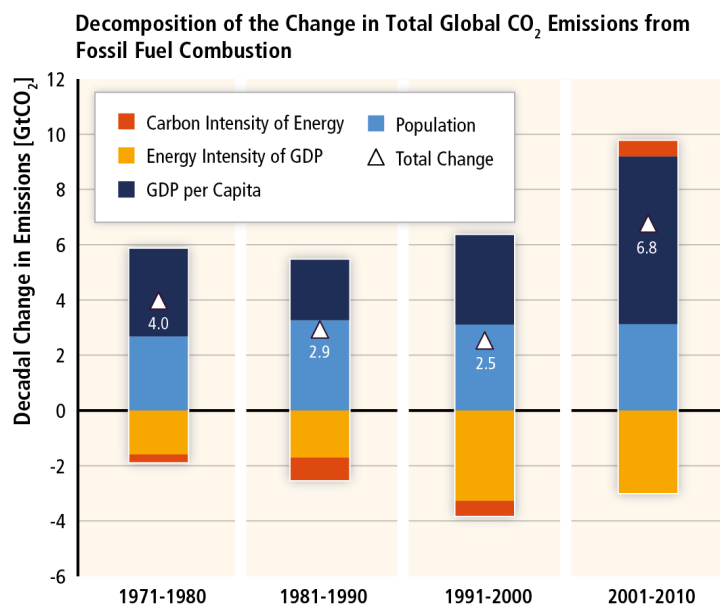
Figure SPM.3. Decomposition of the decadal change in total global CO 2 emissions from fossil fuel combustion by four driving factors; population, income (GDP) per capita, energy intensity of GDP and carbon intensity of energy. The bar segments show the changes associated with each factor alone, holding the respective other factors constant. Total decadal changes are indicated by a triangle. Changes are measured in giga tonnes (Gt) of CO 2 emissions per decade; income is converted into common units using purchasing power parities. [Figure 1.7] [Subject to final quality check and copy edit.]
