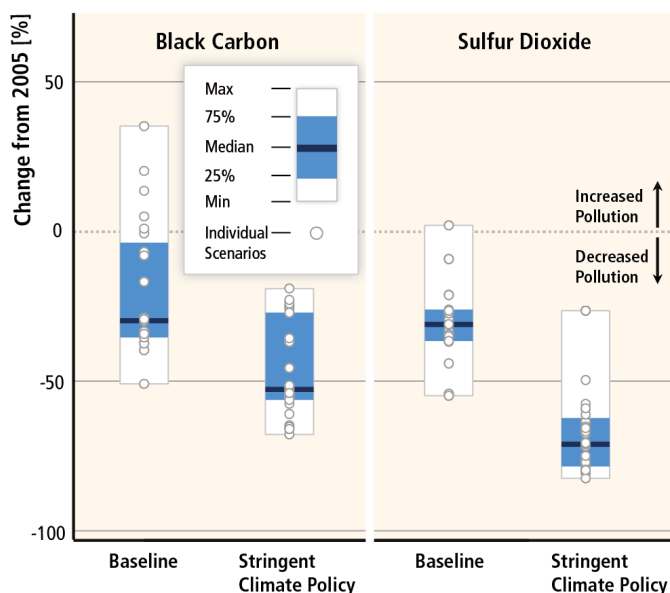
Figure SPM.6. Air pollutant emission levels for black carbon (BC) and sulfur dioxide (SO 2 ) in 2050 relative to 2005 (0=2005 levels). Baseline scenarios without additional efforts to reduce GHG emissions beyond those in place today are compared to scenarios with stringent mitigation policies, which are consistent with reaching atmospheric CO 2 eq concentration levels between 430 and 530 ppm CO 2 eq by 2100. [Figure 6.33] [Subject to final quality check and copy edit.]
