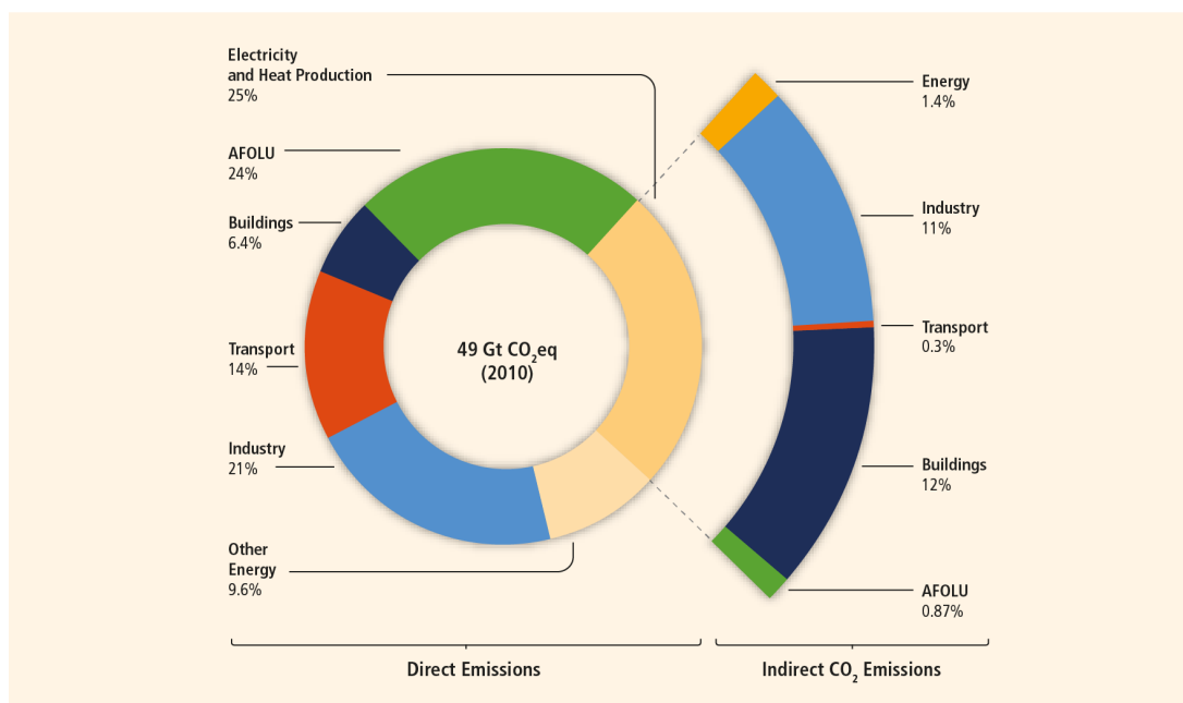
Figure SPM.2. Total anthropogenic GHG emissions (GtCO 2 eq/yr) by economic sectors. Inner circle shows direct GHG emission shares (in % of total anthropogenic GHG emissions) of five economic sectors in 2010. Pull-out shows how indirect CO 2 emission shares (in % of total anthropogenic GHG emissions) from electricity and heat production are attributed to sectors of final energy use. “Other Energy” refers to all GHG emission sources in the energy sector as defined in Annex II other than electricity and heat production [A.II.9.1]. The emissions data from Agriculture, Forestry and Other Land Use (AFOLU) includes land-based CO 2 emissions from forest fires, peat fires and peat decay that approximate to net CO 2 flux from the Forestry and Other Land Use (FOLU) sub-sector as described in Chapter 11 of this report. Emissions are converted into CO 2 -equivalents based on GWP 100 6 from the IPCC Second Assessment Report. Sector definitions are provided in Annex II.9. [Figure 1.3a, Figure TS.3 a/b] [Subject to final quality check and copy edit.]
