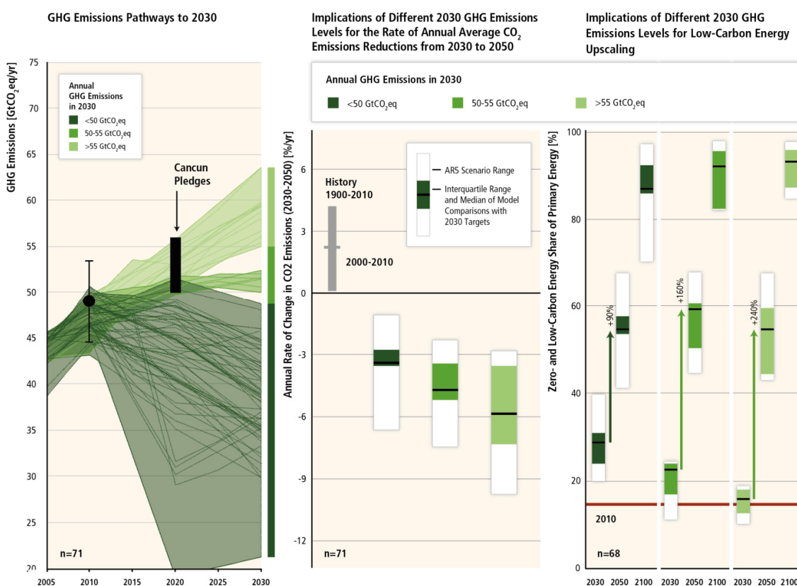
Figure SPM.5. The implications of different 2030 GHG emissions levels for the rate of CO 2 emissions reductions and low-carbon energy upscaling from 2030 to 2050 in mitigation scenarios reaching about 450 to 500 (430–530) ppm CO 2 eq concentrations by 2100. The scenarios are grouped according to different emissions levels by 2030 (coloured in different shades of green). The left panel shows the pathways of GHG emissions (GtCO 2 eq/yr) leading to these 2030 levels. The black bar shows the estimated uncertainty range of GHG emissions implied by the Cancún Pledges. The middle panel denotes the average annual CO 2 emissions reduction rates for the period 2030–2050. It compares the median and interquartile range across scenarios from recent intermodel comparisons with explicit 2030 interim goals to the range of scenarios in the Scenario Database for WGIII AR5. Annual rates of historical emissions change (sustained over a period of 20 years) are shown in grey. The arrows in the right panel show the magnitude of zero and low-carbon energy supply up-scaling from 2030 to 2050 subject to different 2030 GHG emissions levels. Zero- and low-carbon energy supply includes renewables, nuclear energy, and fossil energy with carbon dioxide capture and storage (CCS), or
