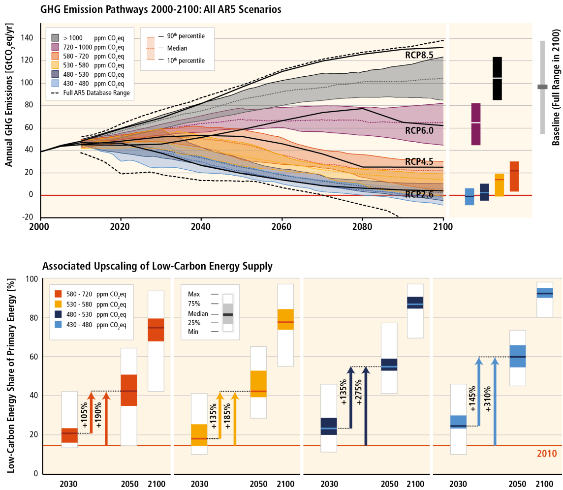
Figure SPM.4. Pathways of global GHG emissions (GtCO 2 eq/yr) in baseline and mitigation scenarios for different long-term concentration levels (upper panel) and associated upscaling requirements of low-carbon energy (% of primary energy) for 2030, 2050 and 2100 compared to 2010 levels in mitigation scenarios (lower panel). The upper and lower panels exclude scenarios with limited technology availability and the lower panel in addition excludes scenarios that assume exogenous carbon price trajectories. [Figure 6.7, Figure 7.16] [Subject to final quality check and copy edit.]
