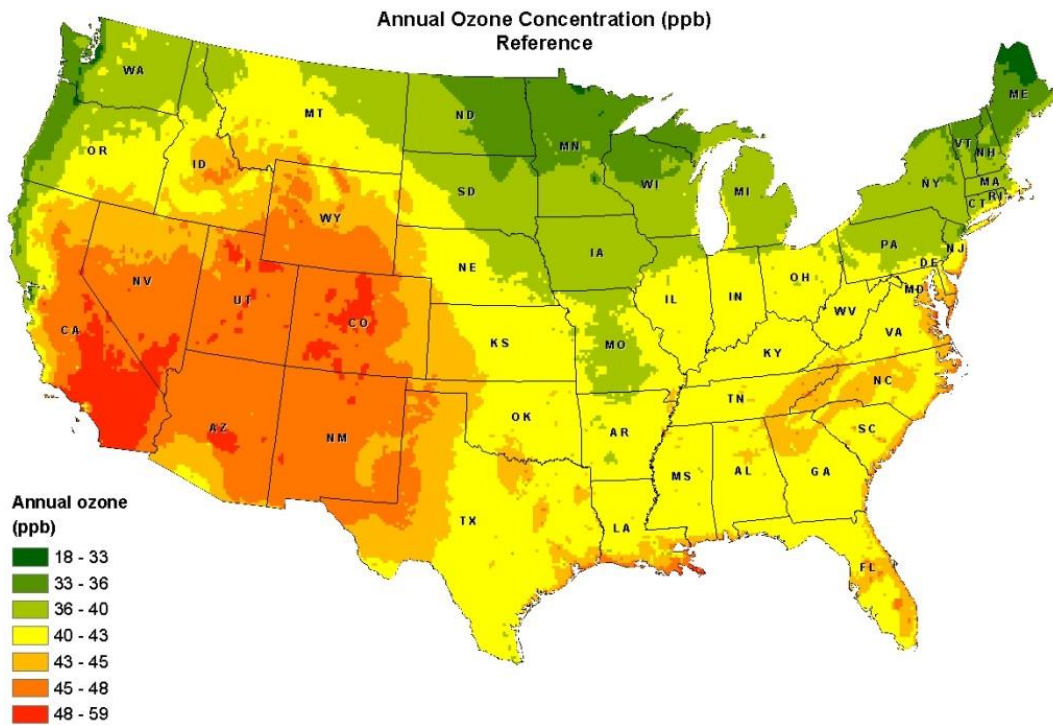
Figure 9a & b: Average annual peak 8-hr ozone for Reference Case and change in this condition for Scenario #2 (parts per billion).
