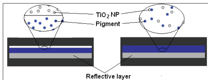
(Left) TiO 2 Layer Coated on Top of the Pigment Layer, and (Right) Shelled TiO 2 Nanoparticles Mixed with the Organic Pigments/Resin
