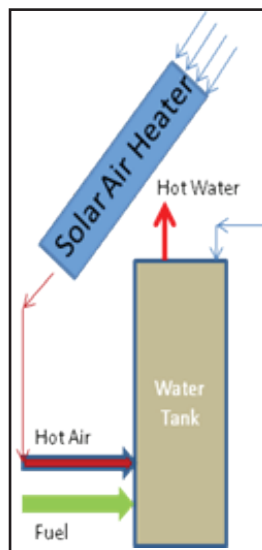
ORNL's Solar Air Heating System
