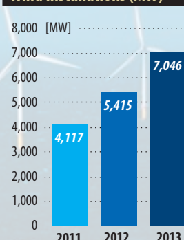
Global Cumulative Offshore Wind Installations (MW)
