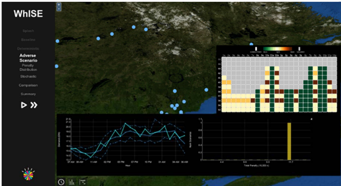
FIGURE 7: WHISE SCREENSHOT
