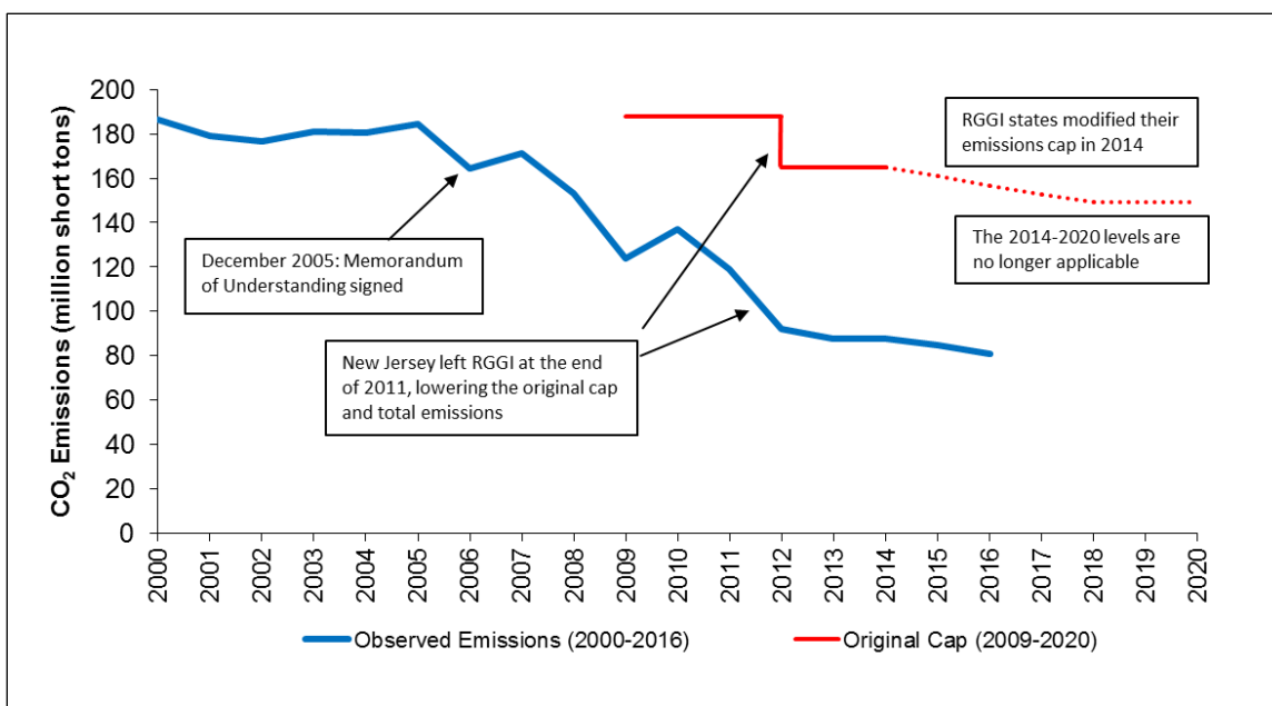
Figure 1. Observed Emissions Compared to the Original Emissions Cap
