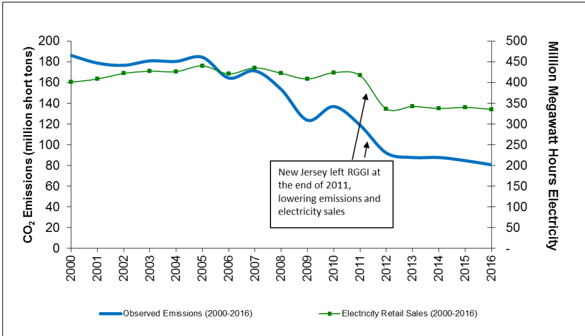
Figure 2. RGGI Emissions Compared with Electricity Sales 2000 - 2016
