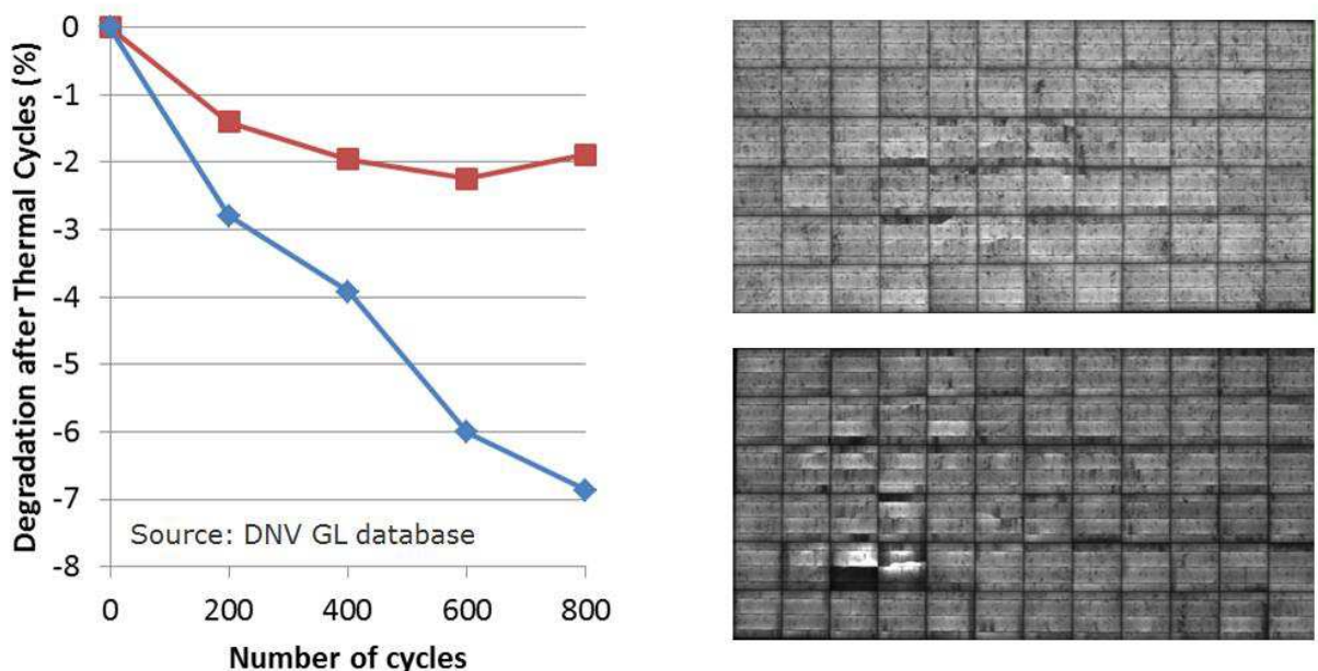
Figure 6-2 Two modules with the same label and a different BOM may perform differently in accelerated tests
