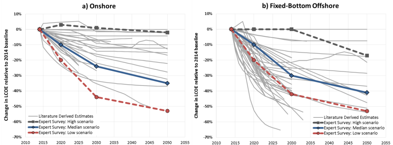
Figure ES-8. Estimated Change in LCOE: Expert Survey Results vs. Other Forecasts
