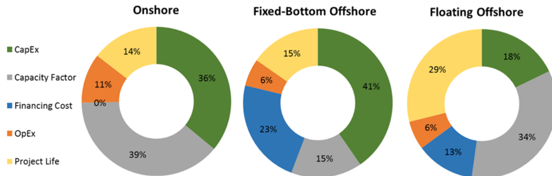
Figure ES-3. Relative Impact of Drivers for Median-Scenario LCOE Reduction in 2030
