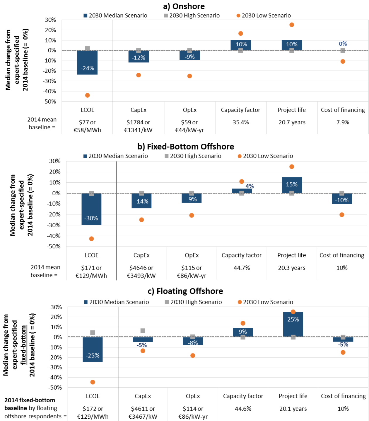
Figure 7. Relative Change in LCOE and LCOE Components from 2014 to 2030 for (a) Onshore, (b) Fixed-Bottom Offshore, and (c) Floating Offshore Wind Projects
