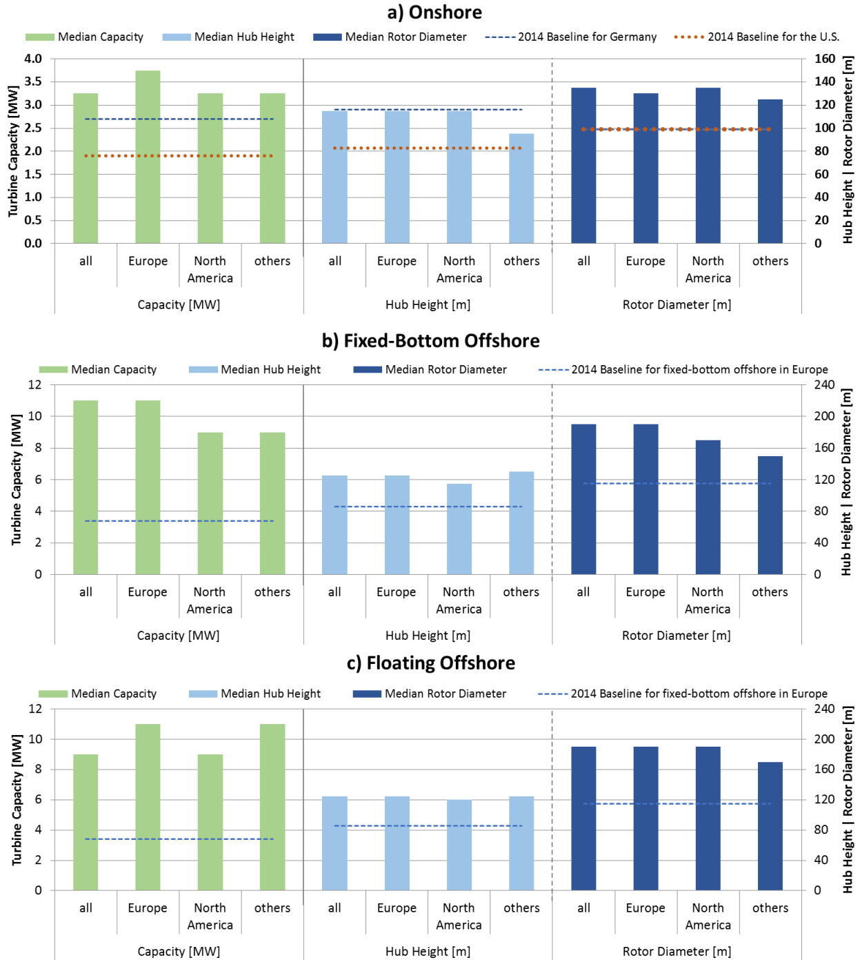
Figure 10. Wind Turbine Characteristics in 2030 for (a) Onshore, (b) Fixed-Bottom Offshore, and (c) Floating Offshore Wind Projects
