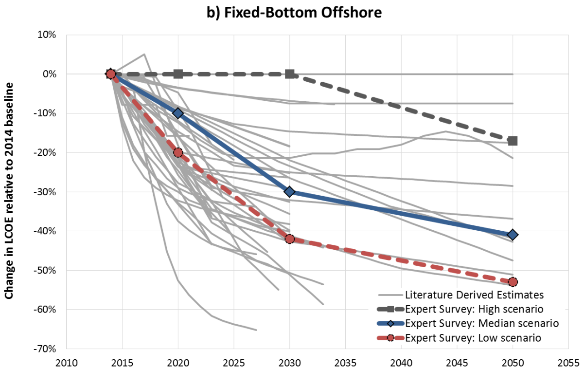
Figure 14. Estimated Change in LCOE over Time for (a) Onshore and (b) Fixed-Bottom Offshore Wind Projects: Expert Survey Results vs. Other Forecasts
