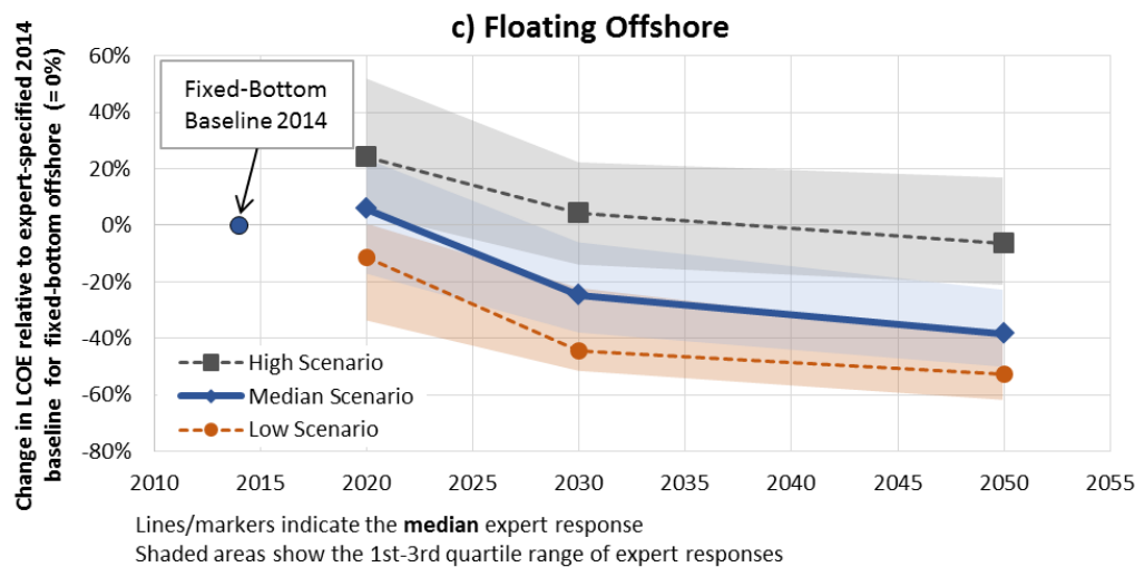
Figure 4. Estimated Change in LCOE over Time for (a) Onshore, (b) Fixed-Bottom Offshore, and (c) Floating Offshore Wind Projects
