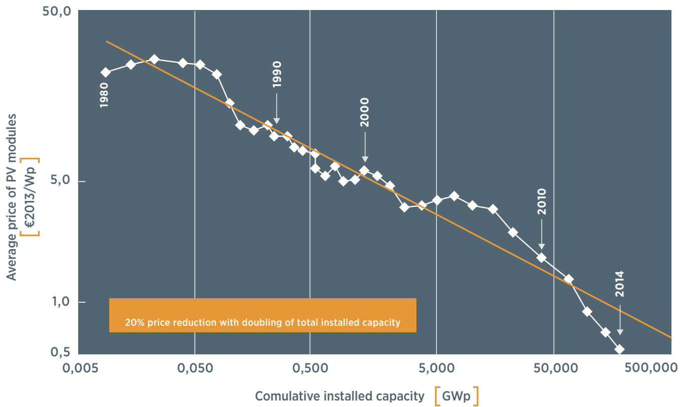
Figure 5.5. Historical price development of photovoltaic modules that relate to the cumulative installed capacity worldwide
