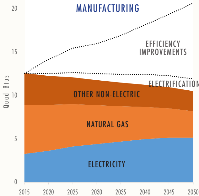
Figure 3-8b. Transformation scenario projections for industry final energy use in manufacturing (left) and non-manufacturing (agriculture, construction, and mining sectors [right]).
