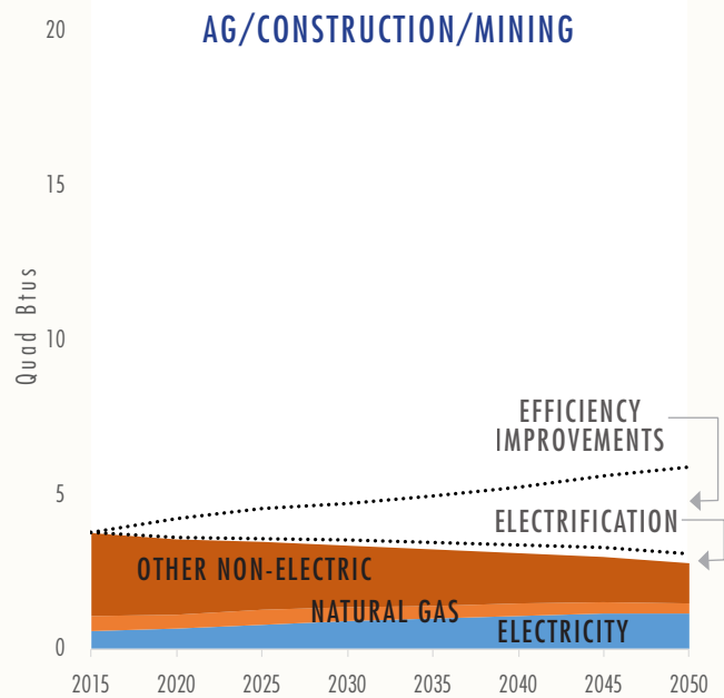
Figure 3-8b. Transformation scenario projections for industry final energy use in manufacturing (left) and non-manufacturing (agriculture, construction, and mining sectors [right]).
