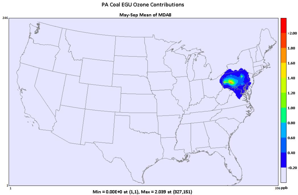
Figure 8-3 Map of Pennsylvania Coal EGU Tag Contribution to Seasonal Average MDA8 Ozone
