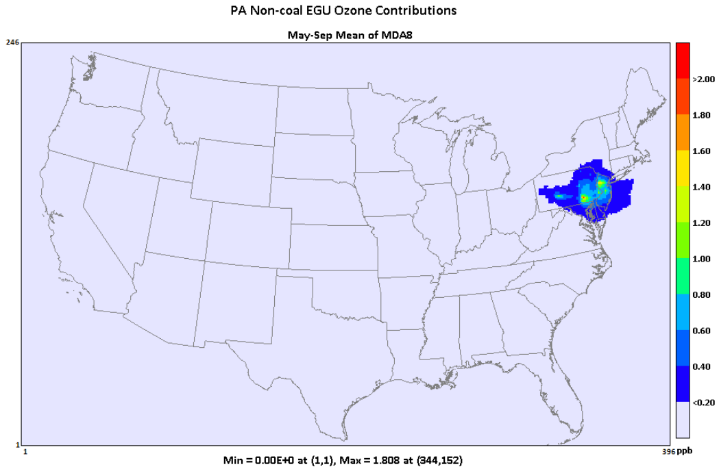
Figure 8-4 Map of Pennsylvania Non-Coal EGU Tag Contribution to Seasonal Average MDA8 Ozone
