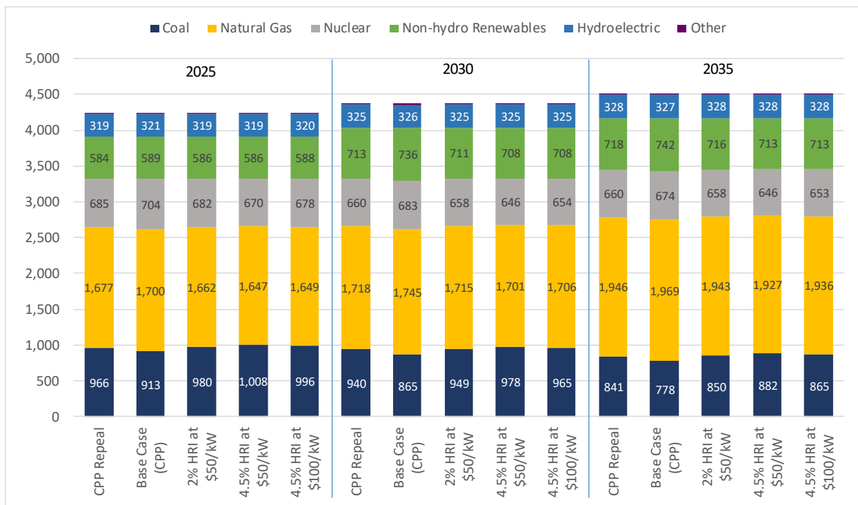
Figure 3-1 Generation Mix (thousand GWh)
