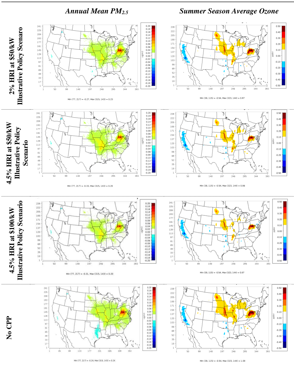
Figure 4-4 Change in Annual Mean PM 2.5 (μg/m 3 ) and Summer Season Average Daily 8hr Maximum Ozone (ppb) in 2025 (Difference Calculated as Illustrative Scenario - Base Case)
