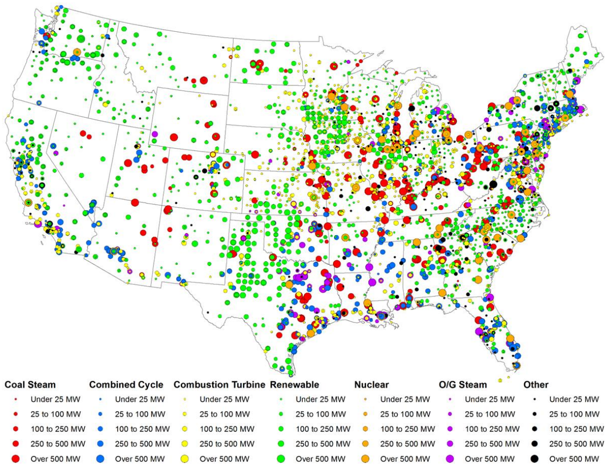
Figure 2-5 Electricity Generating Facilities, by Size and Type
