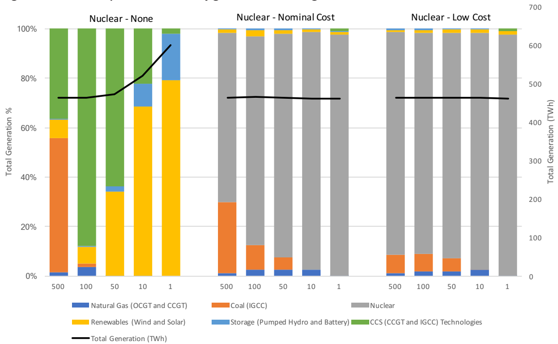
Figure 1.12b: T-B-T dispatchable electricity generation technologies
